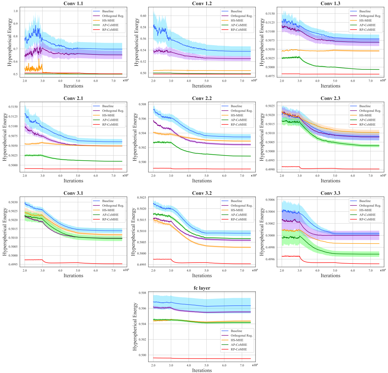
Figure 10: Hyperspherical energy of every layer (Conv1.1, Conv1.2, Conv1.3, Conv2.1, Conv2.2, Conv2.3, Conv3.1, Conv3.2, Conv3.3, fc) after the 20000-th iteration. Note that, all networks are initialized with the same weights and therefore have the same hyperspherical energy at the beginning.
