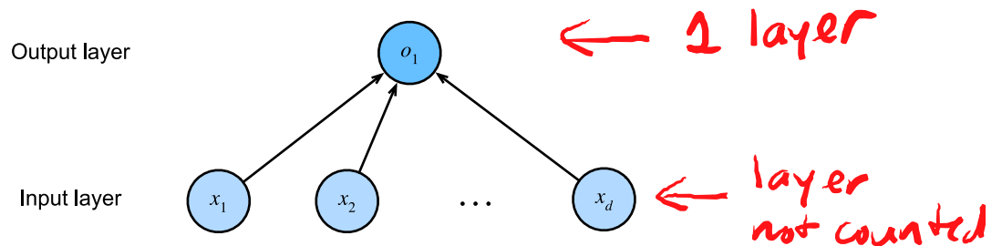
Fig. 3.1.2: Linear regression is a single-layer neural network.
