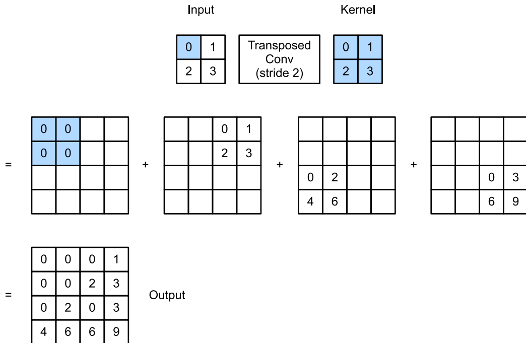
Fig. 13.10.2: Transposed convolution with a 2 \times 2 kernel with stride of 2. The shaded portions are a portion of an intermediate tensor as well as the input and kernel tensor elements used for the computation.
