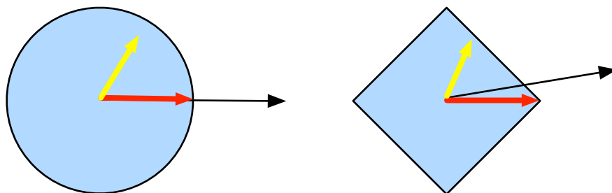
Fig. 11.2.4: Convex Projections.
