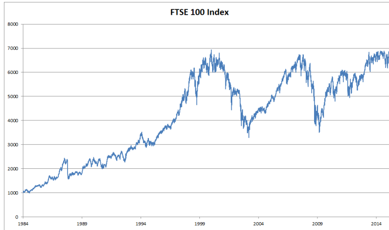
Fig. 8.1.1: FTSE 100 index over about 30 years.
