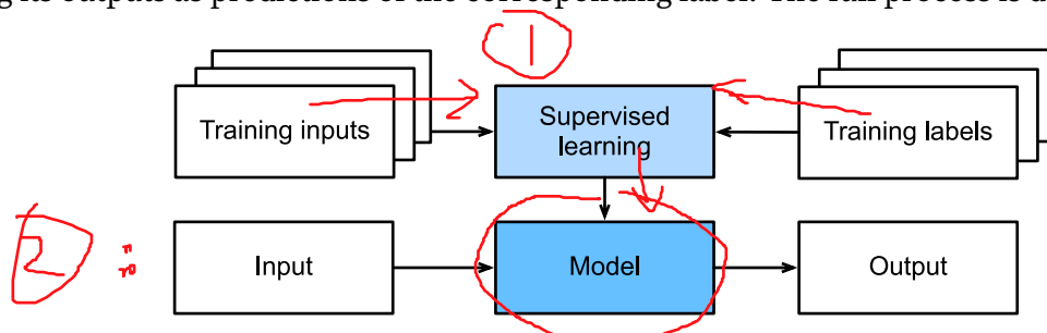
Fig. 1.3.1: Supervised learning.
