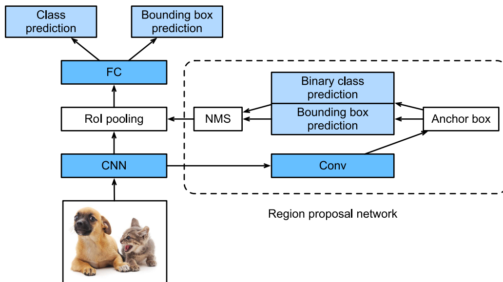
Fig. 13.8.4: The faster R-CNN model.
