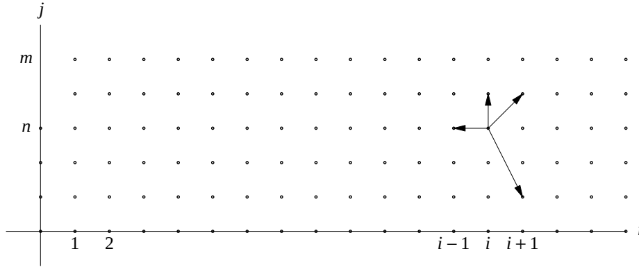
Figure 1: State space of an M/M/1 type model
