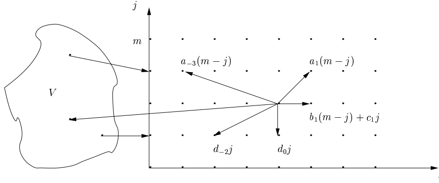
Figure 1: Transition rate diagram for the G/M/1 type model with linear rates
