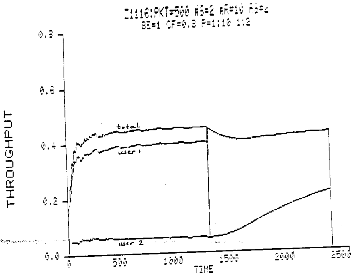
Figure 1: Non-selective bit setting - unfairness with different paths
