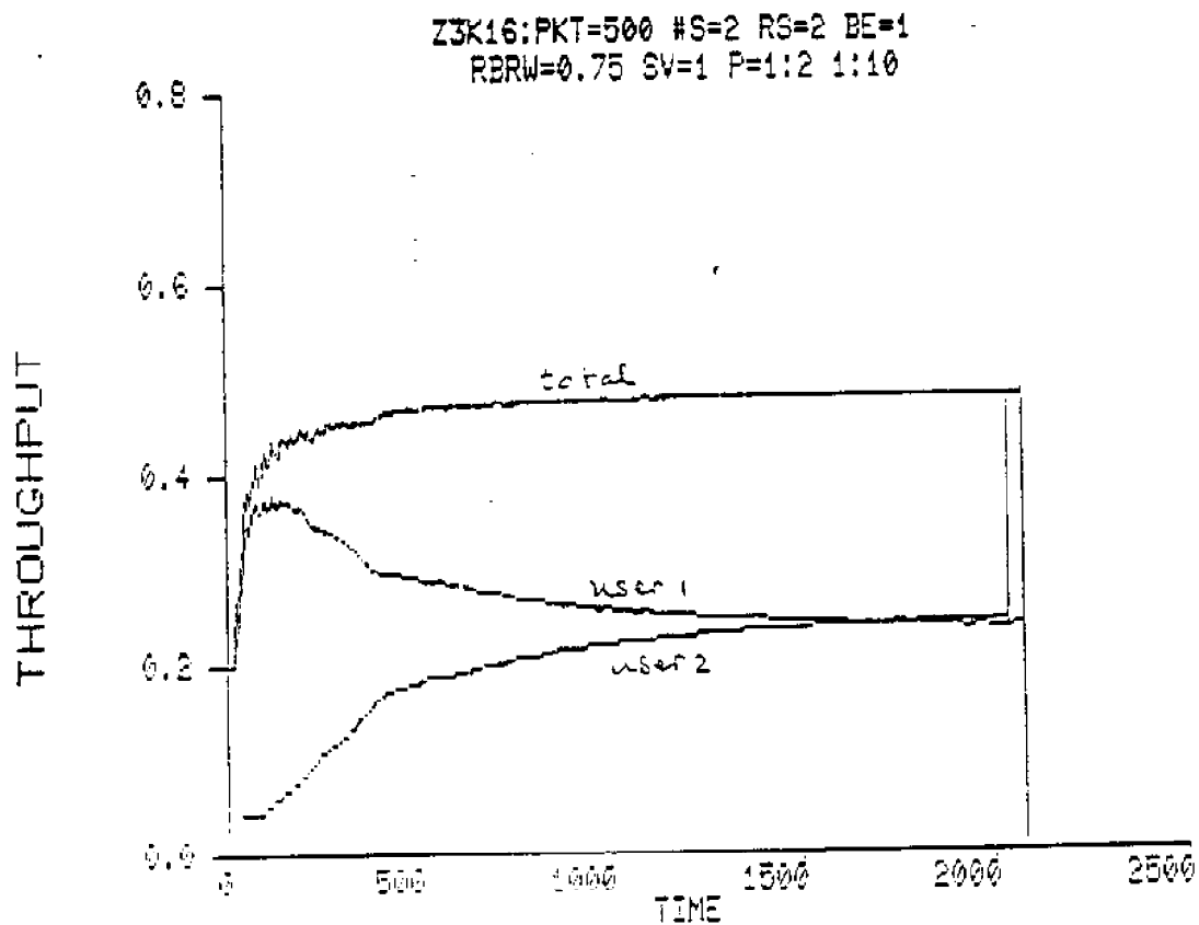
Figure 7: Throughput with Multiple Users, Capacity Factor=0.9, Configuration 1.
