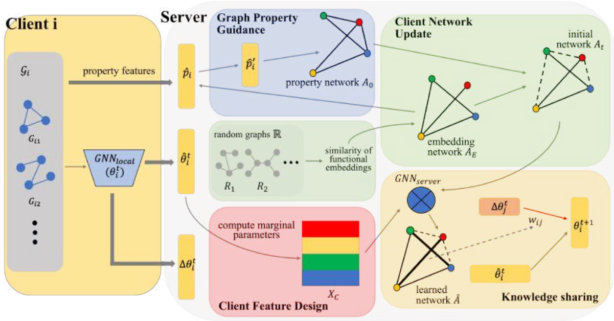
Figure 2: Overview of GPFL. Knowledge sharing is performed under the guidance of the client network, which is reconstructed from marginal parameters. The initialization of this network is guided by fundamental graph properties and functional embeddings to ensure consistent federated collaboration.
