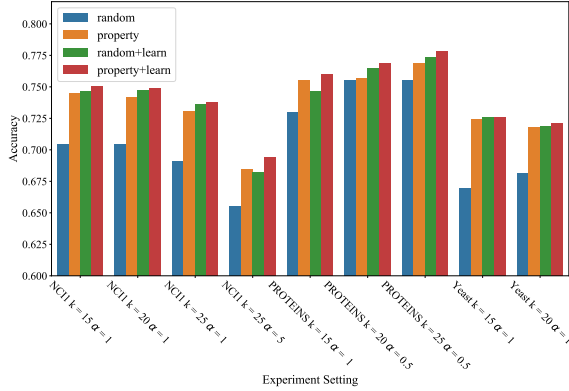
Figure 4: Ablation Study of GPFL.
