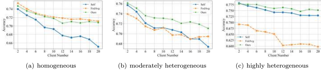
Figure 1: Experimental analysis on the influence of data heterogeneity over FL on a real-world graph dataset (NCI1 Morris et al. (2020)). Clients within the same group share consistent label distributions while the heterogeneity between groups grows as the setting changes from homogeneous to highly heterogeneous.
