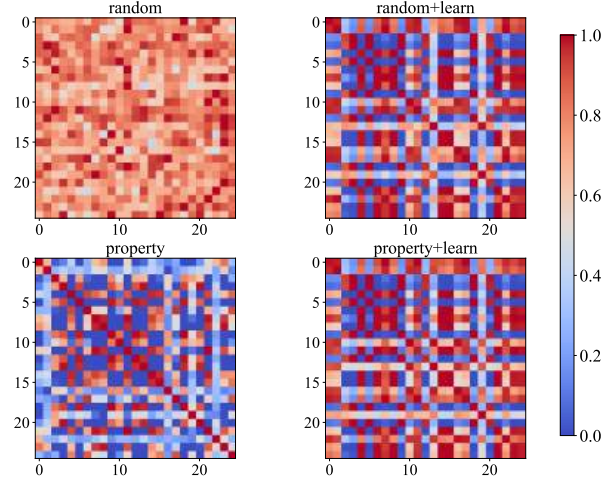
Figure 5: Client Network Visualization on NCI1 dataset with 25 clients and \alpha = 0.5 .
