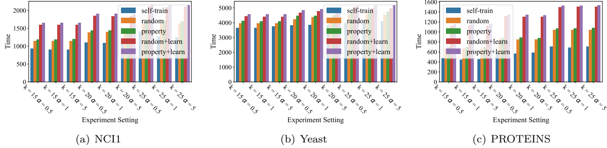
Figure 6: Run time analysis on property-based initialization and network learning.
