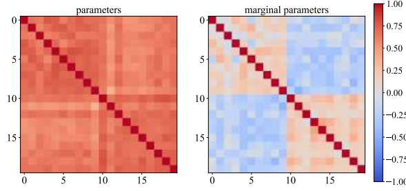
Figure 3: Similarity of local parameters and marginal parameters under high heterogeneity.
